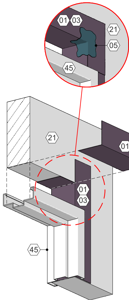
Rough Opening with Adhered Flashing
