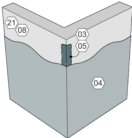
3 Outside Corner, Continuous Liquid AWB
