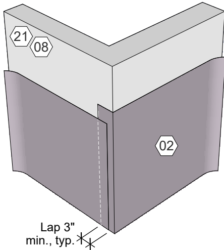
1 Outside Corner, Continuous Adhered AWB
