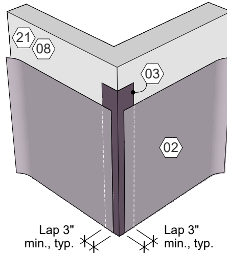
2 Outside Corner, Adhered AWB w/ Flashing Strip
