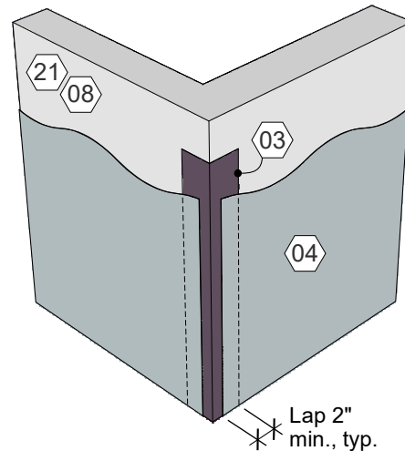
4 Outside Corner, Liquid AWB w/ Flashing Strip
