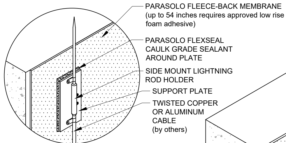
ALTERNATE ROD WALL MOUNT
