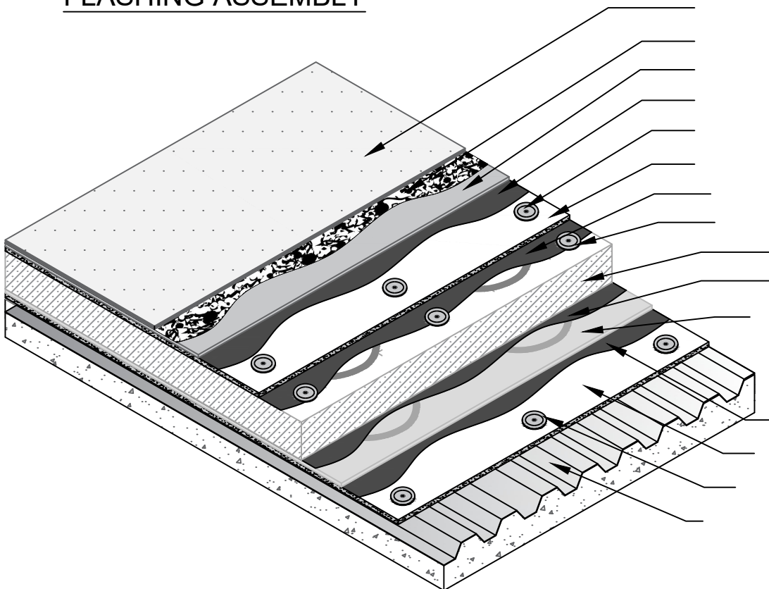
ROOF ASSEMBLY
