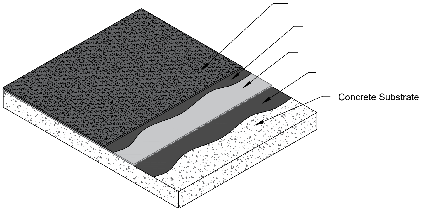
ROOF ASSEMBLY
