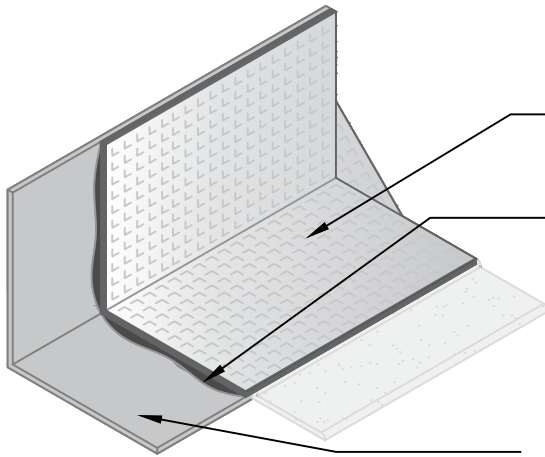
FLASHING ASSEMBLY
