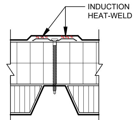
PLATE WELDED DETAIL
