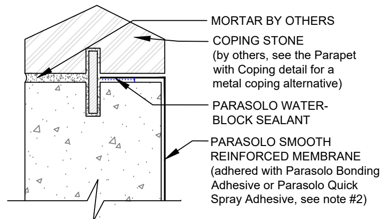
4. COPING STONE TERMINATION
