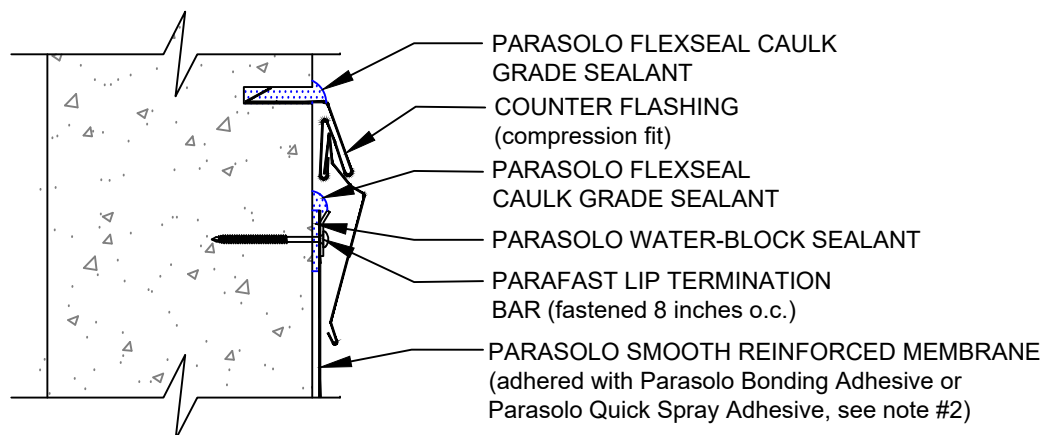
1. REGLET COUNTER FLASHING TERMINATION
